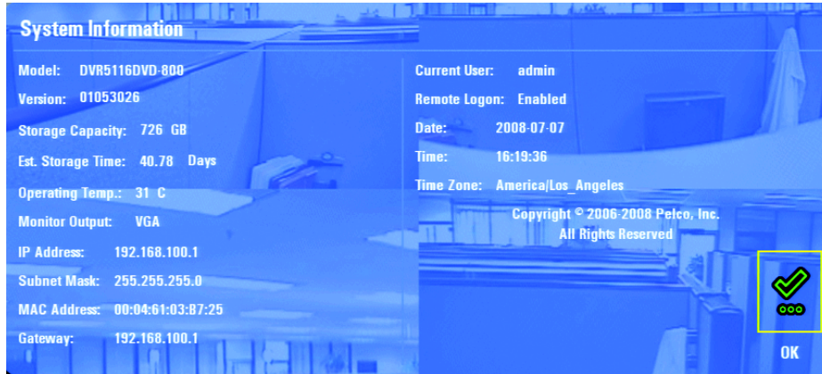
Figure 11. System Information
